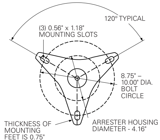
Figure 3. Mounting base details.
