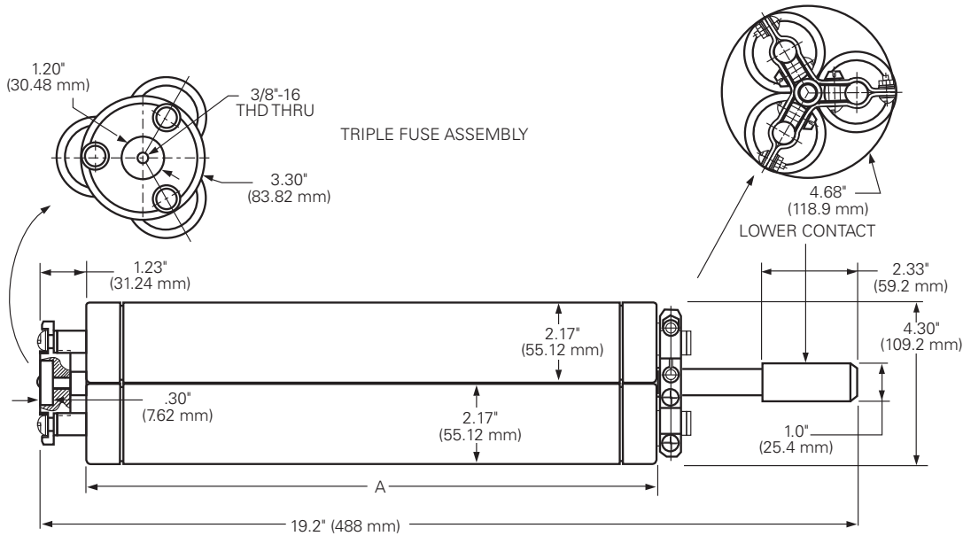
Figure 10. Dimensional information for E-rated 15.5 kV (150E) version ELSG fuses - 25 kV & 35 kV Wetwell Holder
