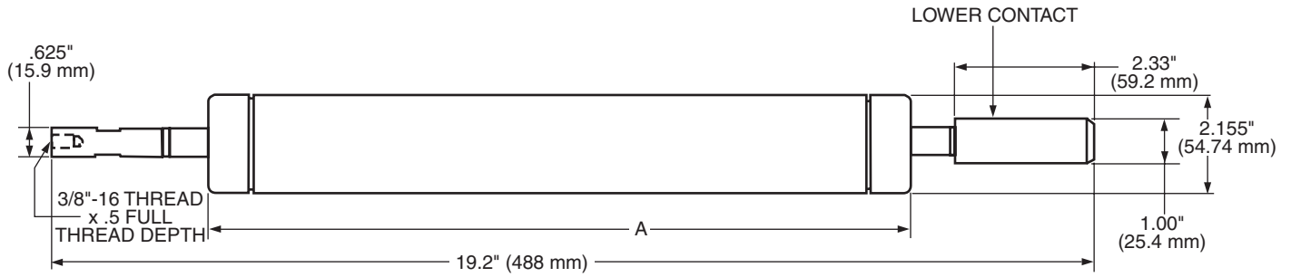
Figure 3. Dimensional information for single 2" diameter 8.3 kV and 15 kV E-rated and MSLE version ELSG fuses
