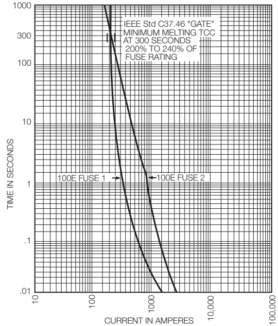
Figure 2. 100E rated current-limiting fuse "gate" per IEEE®
