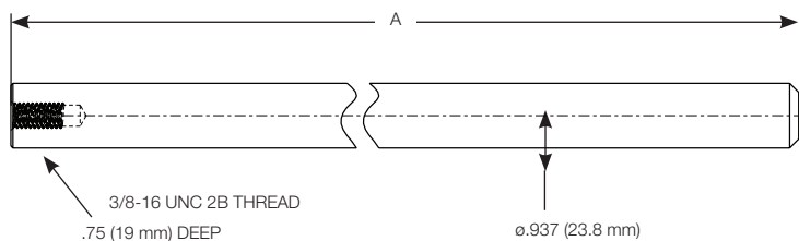
Figure 15. Dimensional Information for shorting bar
