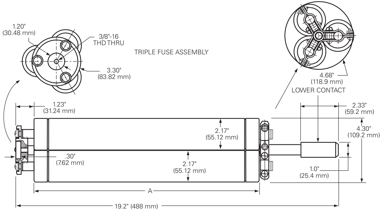
Figure 6. Dimensional information for E-rated 15.5 kV (150E) version ELSG fuses - 15 kV Wetwell Holder
