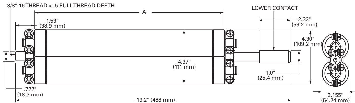
Figure 9. Dimensional information for E-rated 23 kV (50E, 65E) and 15.5 kV and 23 kV (90A) MSLE version ELSG fuses
