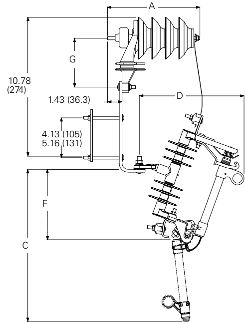
Figure 12. UltraSIL polymer-housed surge arrester/ UltraSIL polymer-insulated Type L fuse cutout/arrester combination— dimensions in inches (mm)
