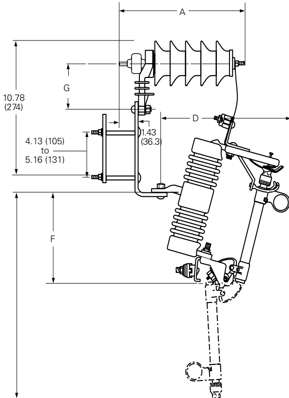
Figure 11. UltraSIL polymer-housed surge arrester/porcelain Type L fuse cutout/arrester combination—dimensions in inches (mm)
