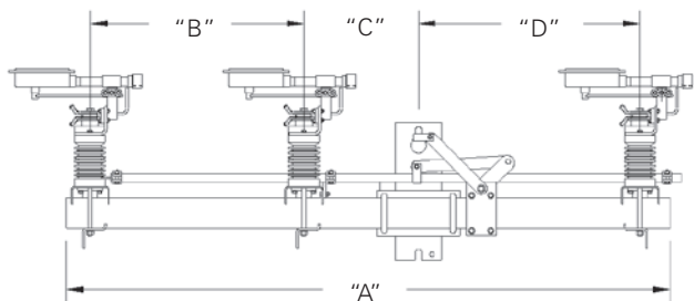
Figure 4. Horizontal switch configuration.
