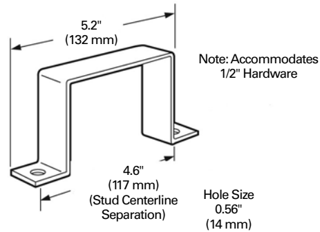
Figure 3. Stainless steel "U" strap for direct wall mount.
