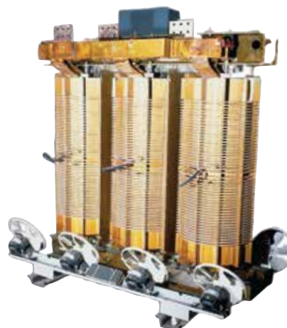
Completed Core and Coil assembly shown with optional fan cooling
