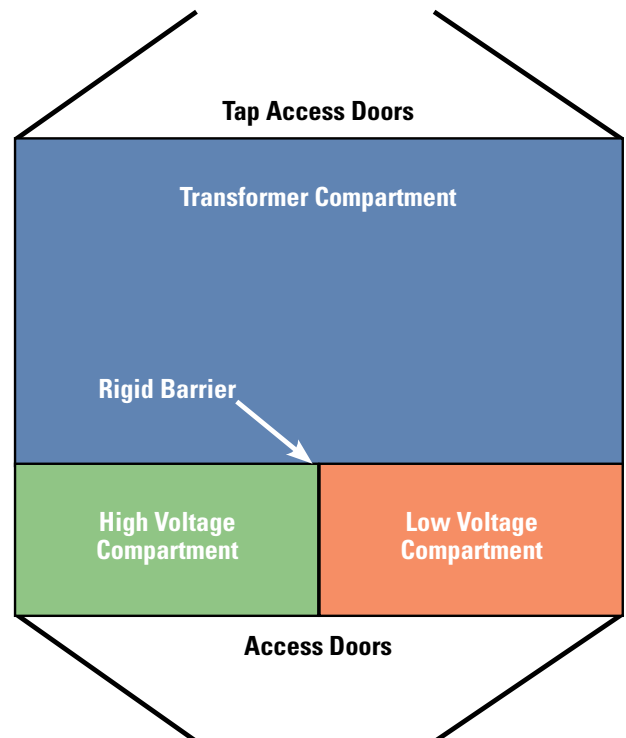
Overhead view of Federal Pacific's Pad-mounted Transformer.
