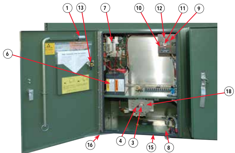
Figure 5. Interior of Run-and-Trip motor operator.
