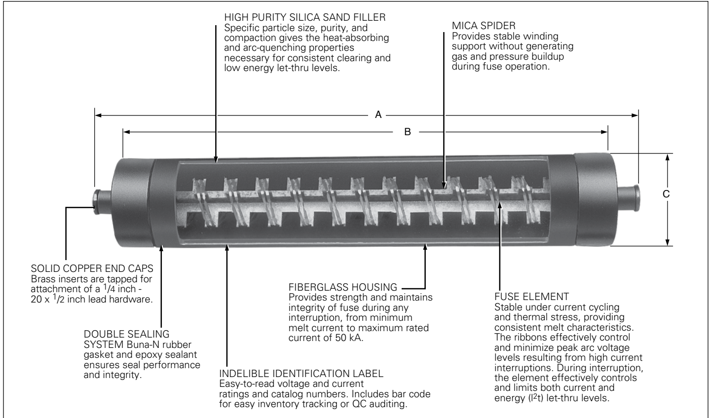
Figure 1. 2 inch diameter ELSP current-limiting backup fuse cutaway shows design characteristics
